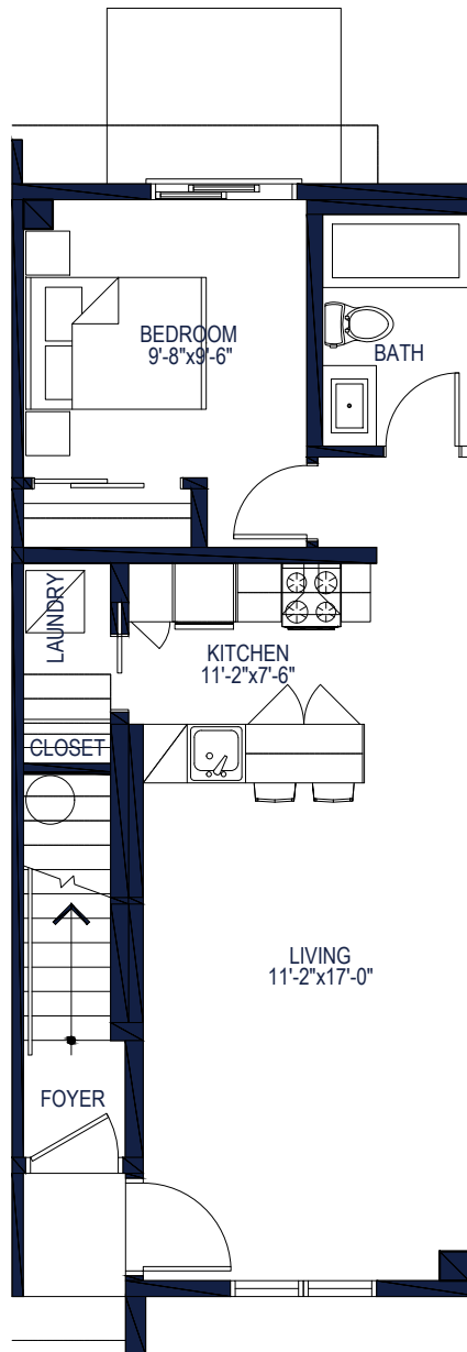
^ Main Level
